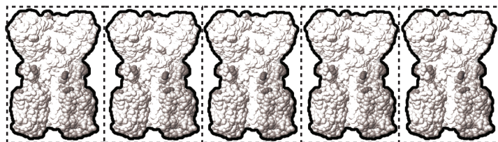
ACE2 protein
