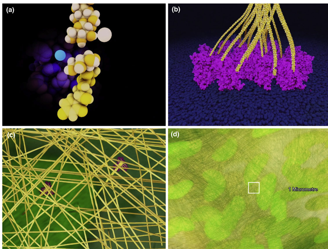
Fig. 4. An animation by Drew Berry presents a continuous zoom from atoms to an entire plant. Four frames from the mesoscale portion of the film are shown here: nanoscale views of (a) cellulose and (b) cellulose synthase, and (c, d) microscale views of the cell wall, with chloroplasts visible through a translucent cell membrane. Images kindly provided by Drew Berry.
