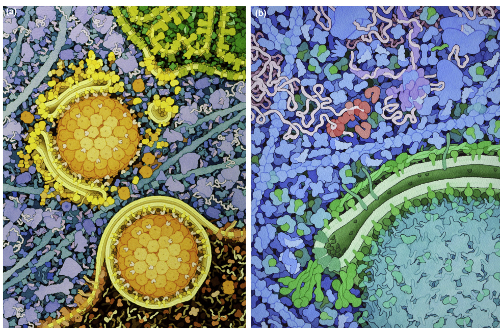
Fig. 7. Illustrations of the “cytoplasm to vacuole targeting” (Cvt) process of autophagy, created in a collaboration with Daniel Klionsky. (a) The first illustration was created in 2006 and includes simple representations of the many proteins orchestrating the formation of the phagophore. (b) In 2014, new data allowed more detailed representation of the proteins and complexes.
