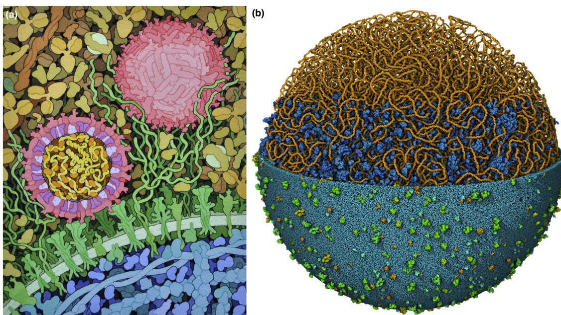
Fig. 1. Mesoscale illustrations. (a) Hand-drawn illustration of Zika virus recognizing a target cell, created for educational outreach at the RCSB Protein Data Bank ( http://pdb101.rcsb.org ). (b) Three-dimensional model of a full mycoplasma cell. The DNA is modeled using lattice-based methods [22], the membrane with LipidWrapper [23], and the remaining molecules with CellPACK [24]. The model is visualized in CellView [25], using selective clipping to progressively reveal the interior molecules (center) and only the DNA (top). Mycoplasma illustration created by Ludovic Autin.
